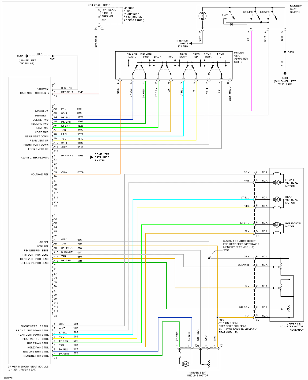
Fig. 33: Memory Systems Circuit
