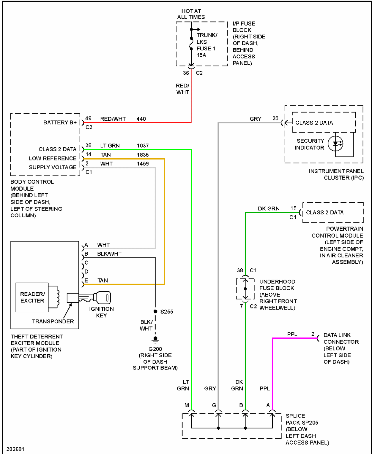
Fig. 8: Pass-Key Circuit
