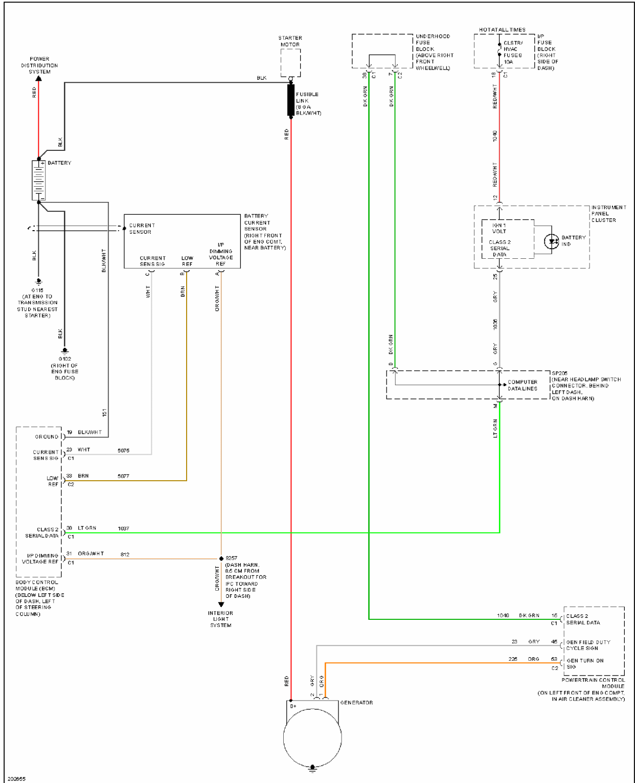
Fig. 52: Charging Circuit
