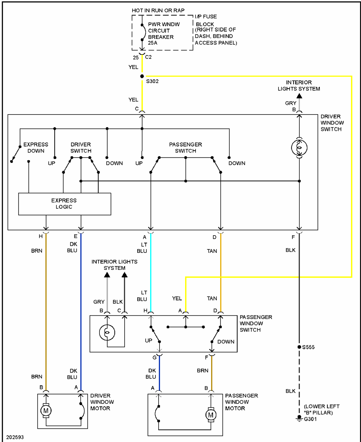
Fig. 46: Power Windows Circuit
