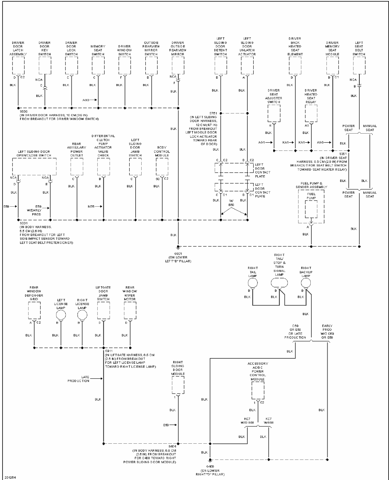
Fig. 24: Ground Distribution Circuit (3 of 5)
