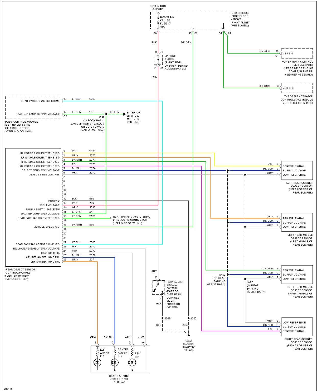
Fig. 34: Parking Assistant Circuit
