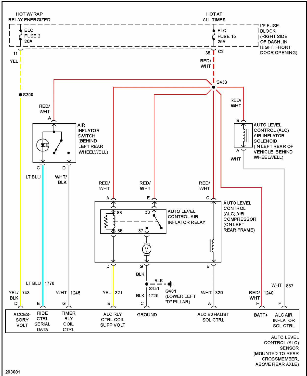
Fig. 14: Electronic Suspension Circuit
